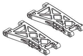
Rear Lower Susp. Arm(AL)
